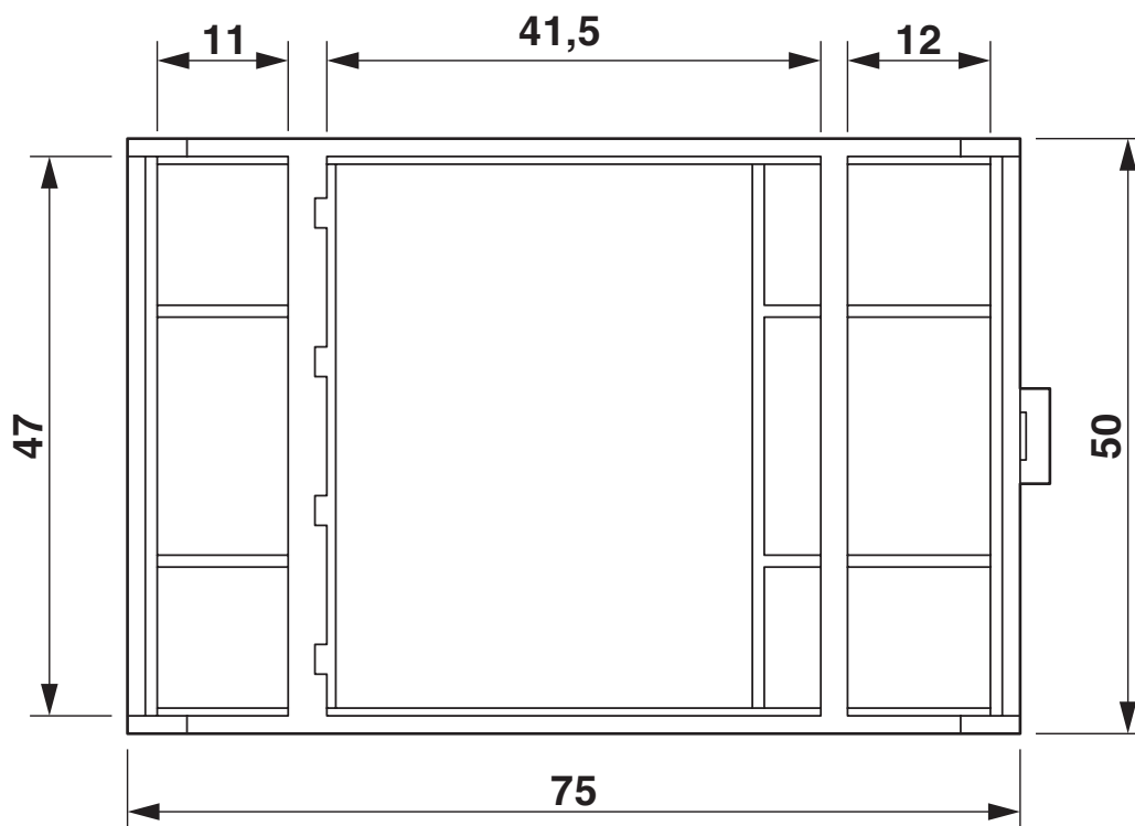
Dimensional drawing
