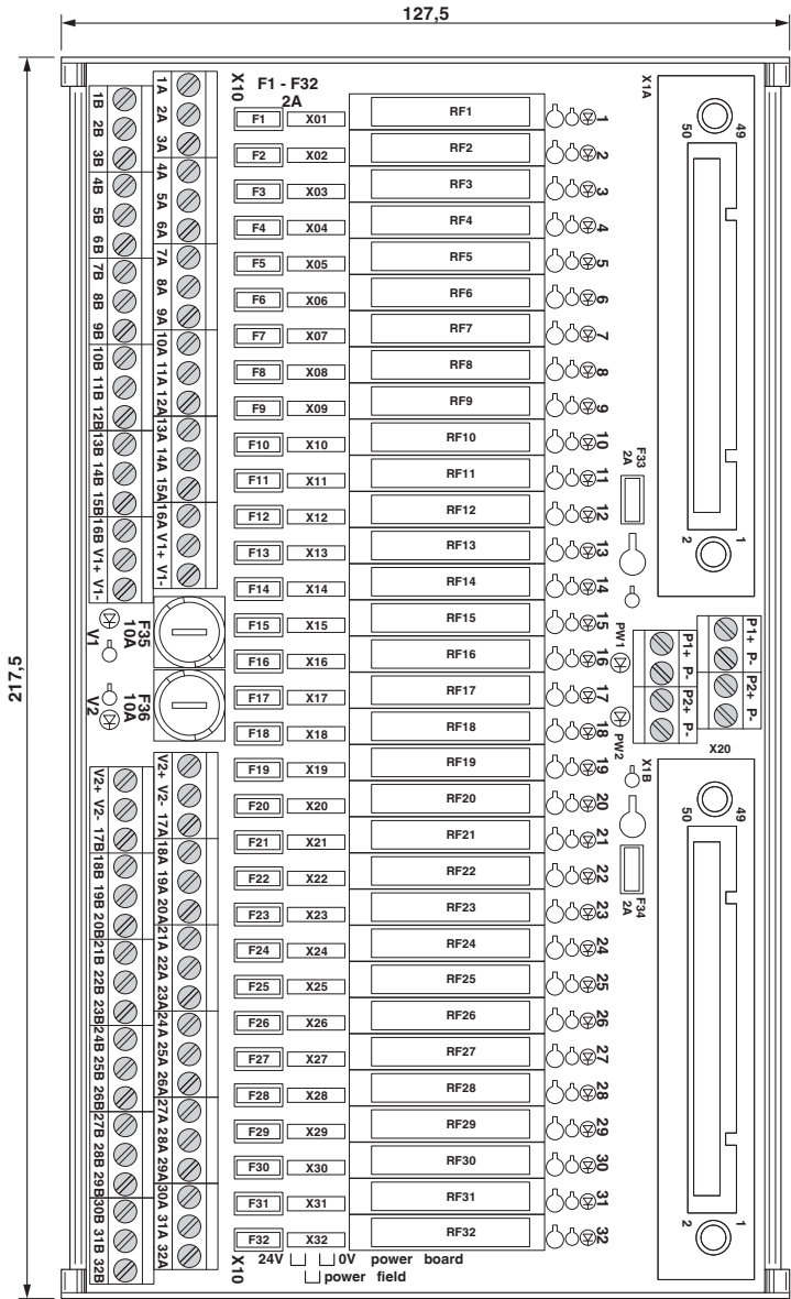
Dimensional drawing
