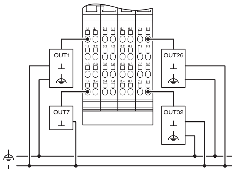
Connection diagram
