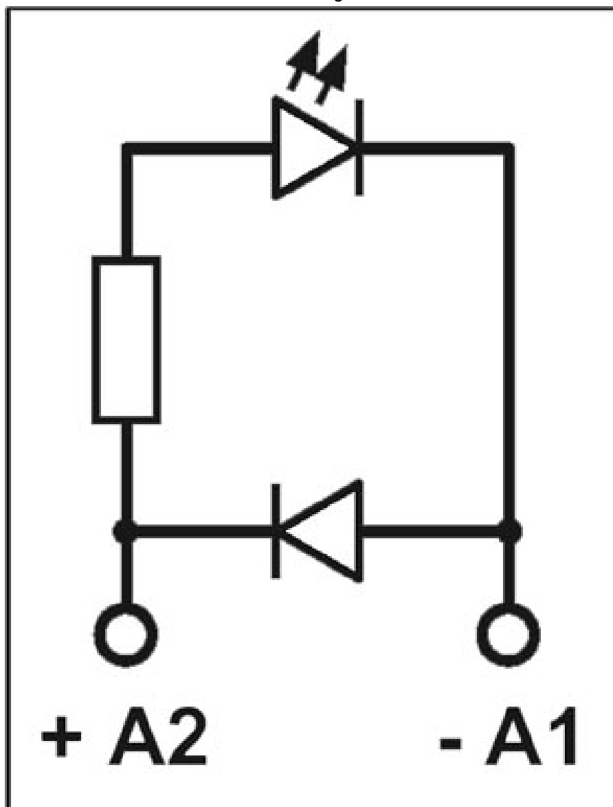
Circuit diagram
