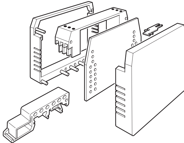
Exploded view
