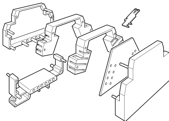
Exploded view
