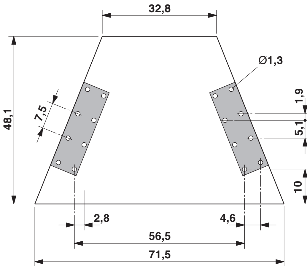
Dimensional drawing
