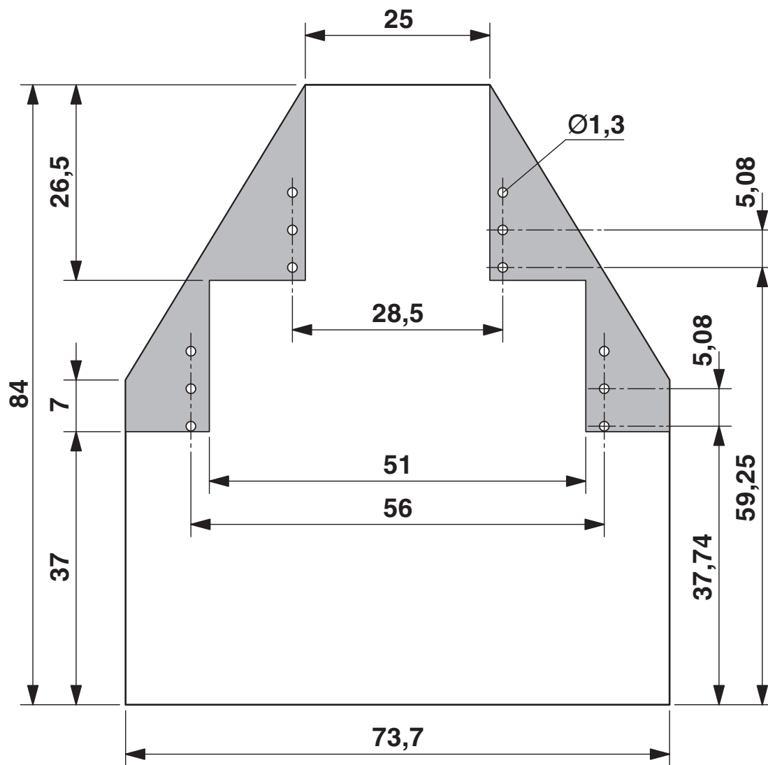
Dimensional drawing
