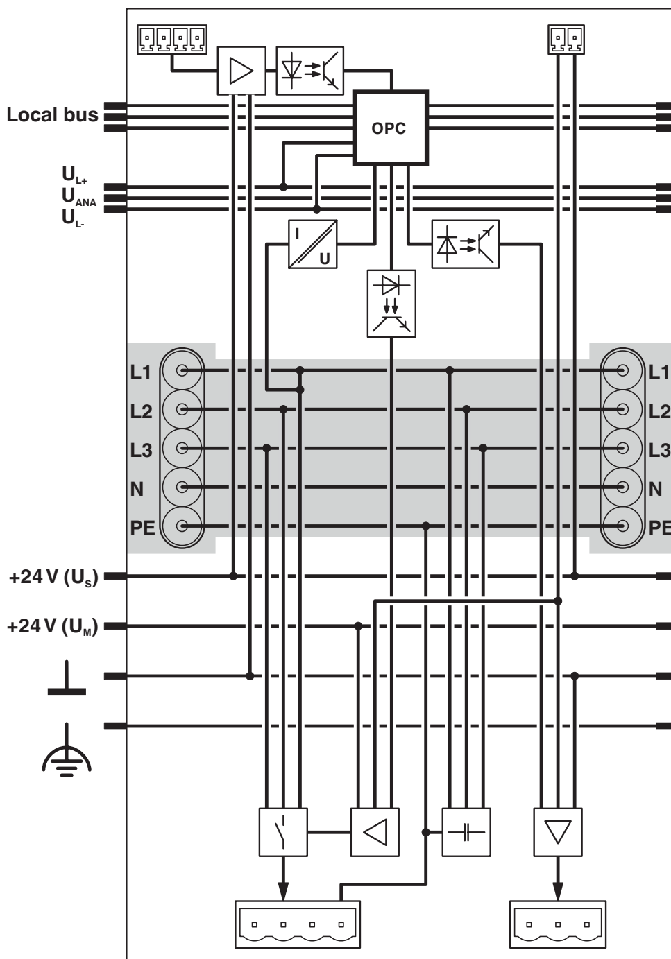
Block diagram
