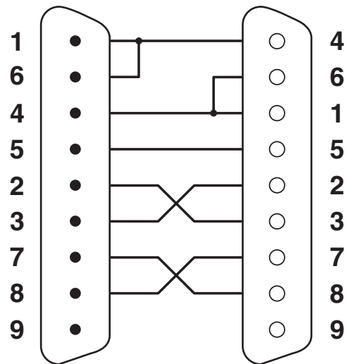
Circuit diagram
