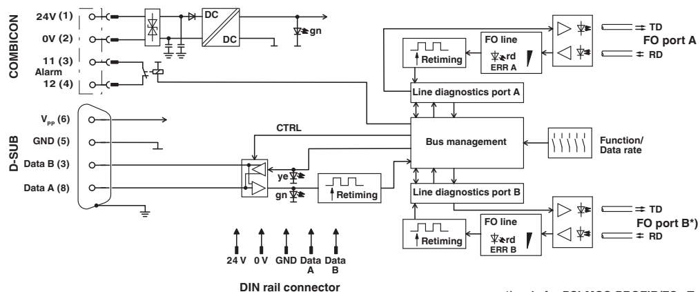
Block diagram
