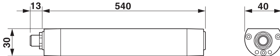
Dimensional drawing
