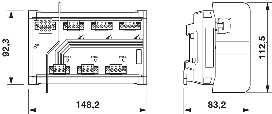
Dimensional drawing
