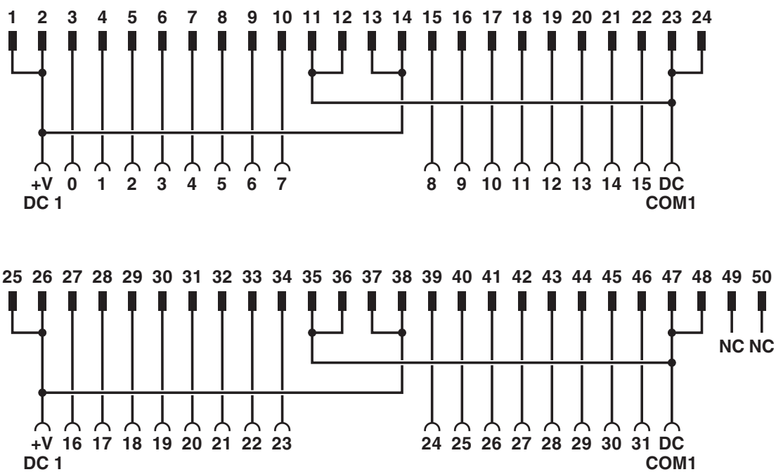
Circuit diagram
