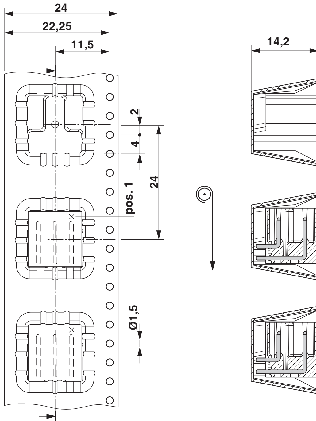
Dimensional drawing
