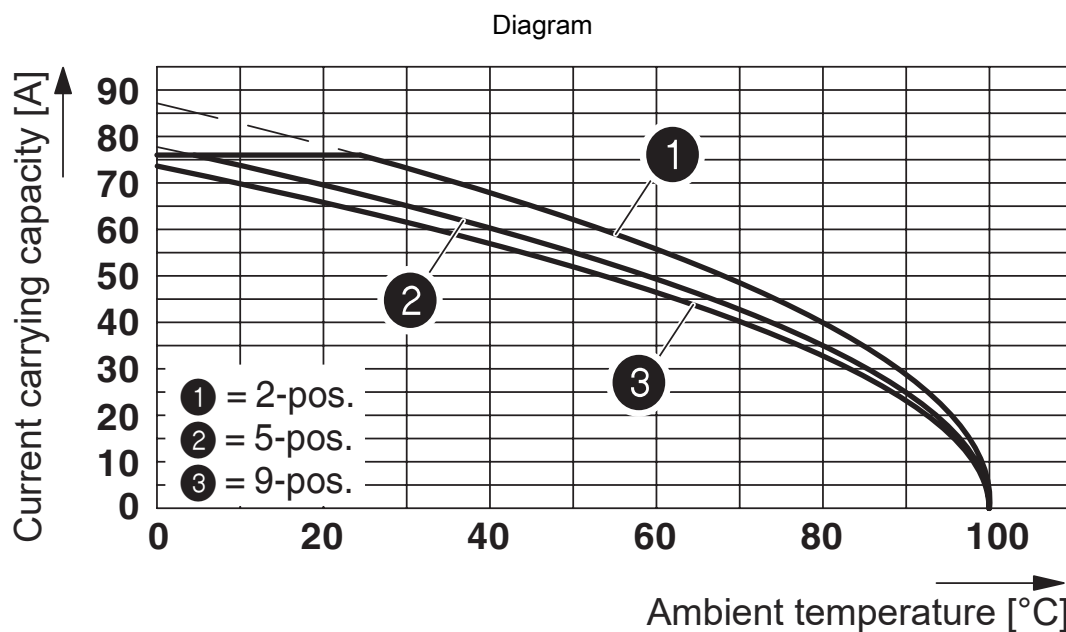
The figure shows the derating curve for DFK-IPC 16/...-G-10,16 inverted plugs in combination with the inverted header IPC 16/...-ST-10,16.
