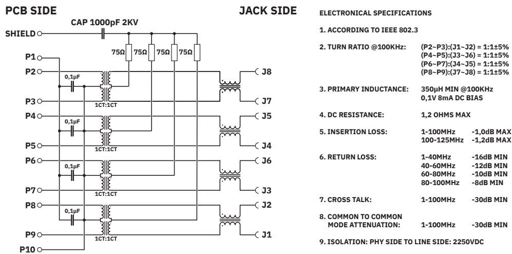
Circuit diagram
