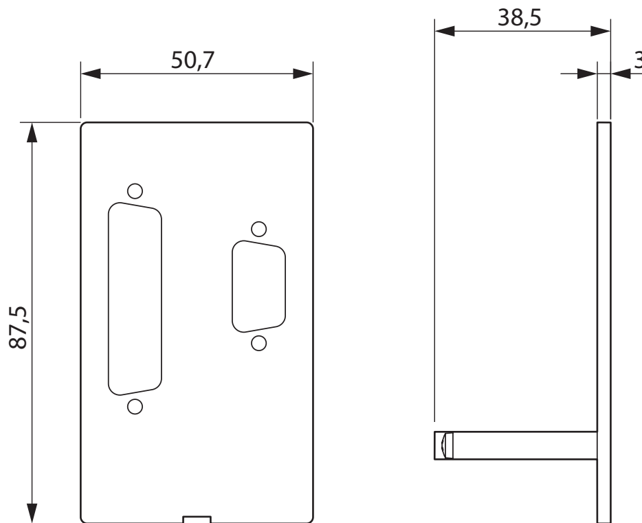
Dimensional drawing
