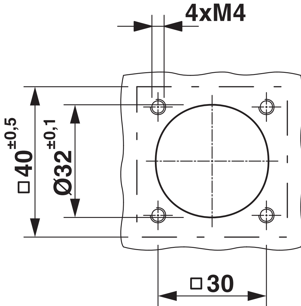
Dimensional drawing
