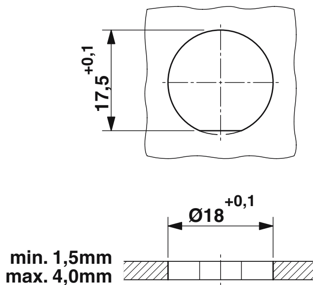
Dimensional drawing
