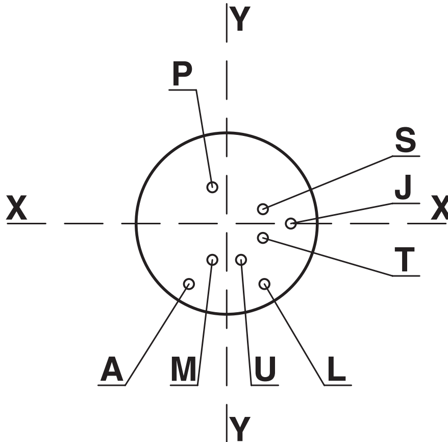
Schematic diagram
