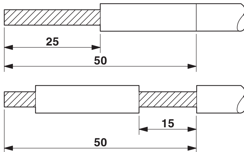
Functional drawing
