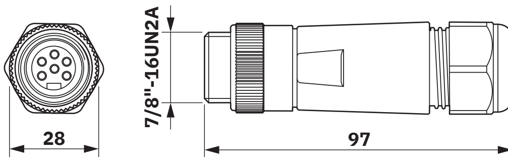
Dimensional drawing
