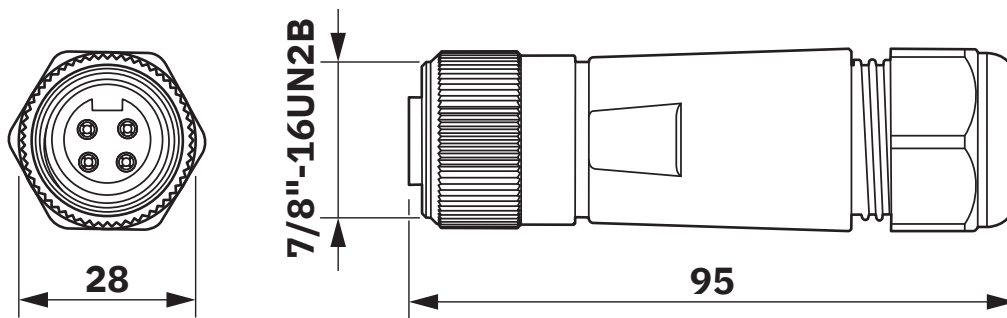
Dimensional drawing
