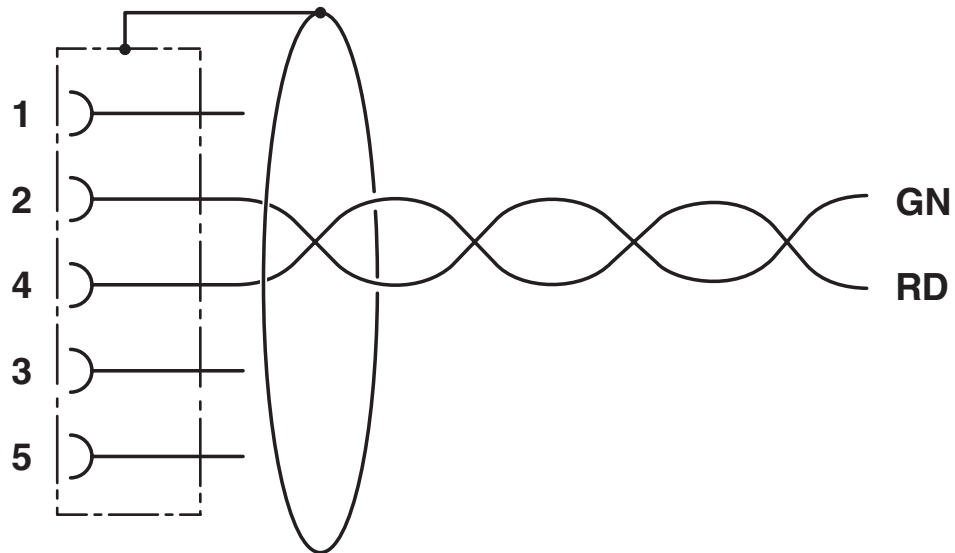
Circuit diagram
