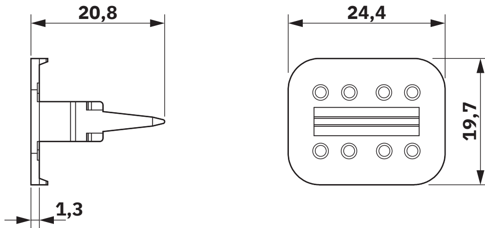
AW8S top view and side view
