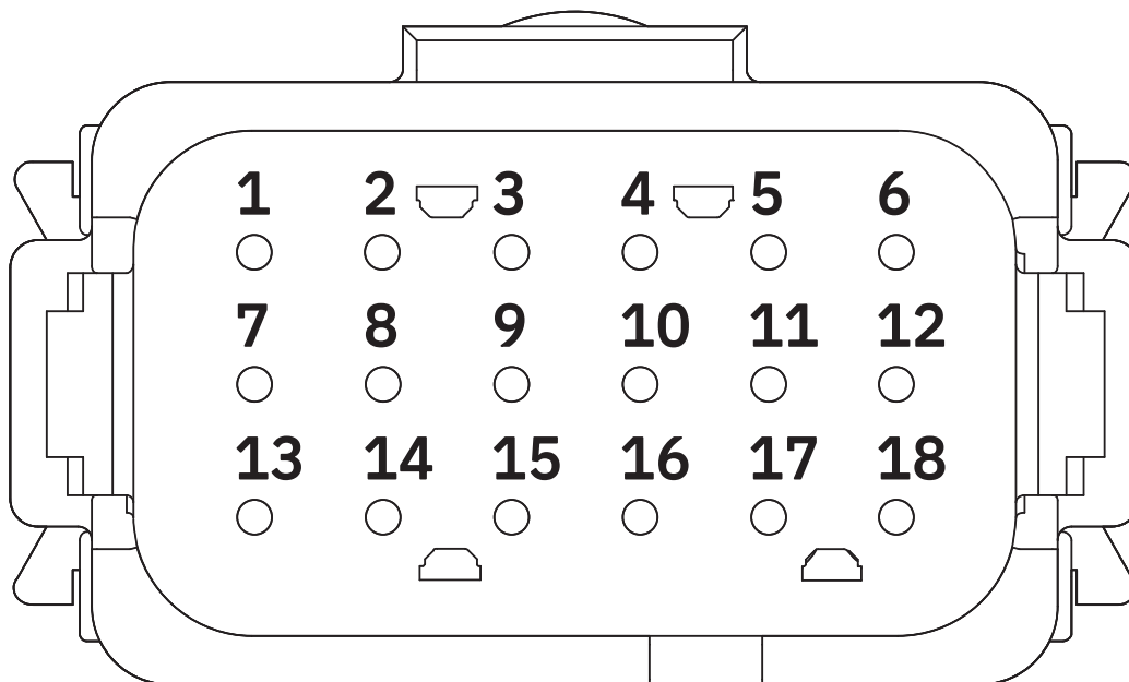
AT16-18PA pin assignment
