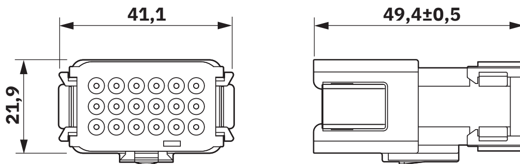
AT16-18PA top view and side view
