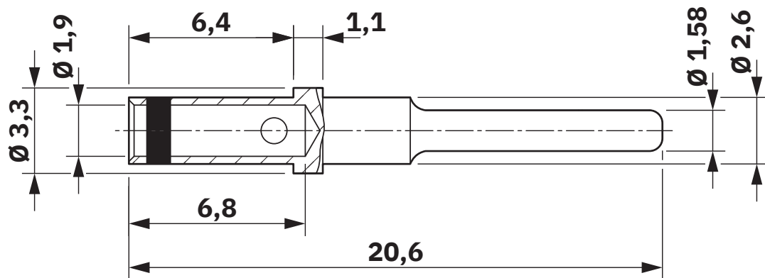
Dimensional drawing
