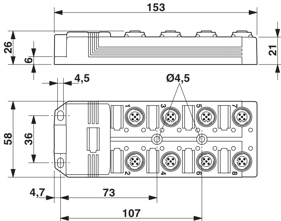
Dimensional drawing
