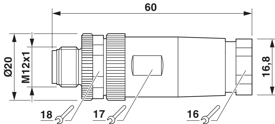
Dimensional drawing
