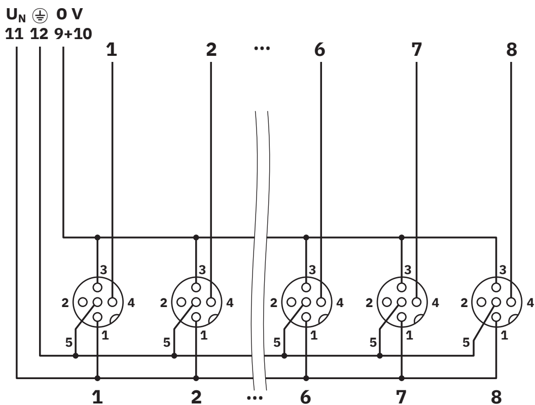
Circuit diagram
