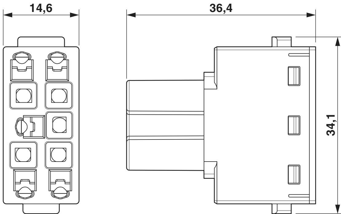
Dimensional drawing
