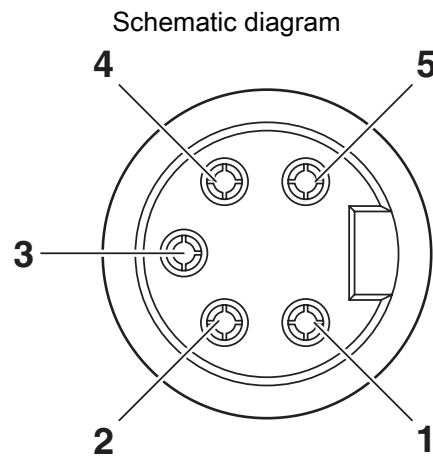
Circuit diagram
