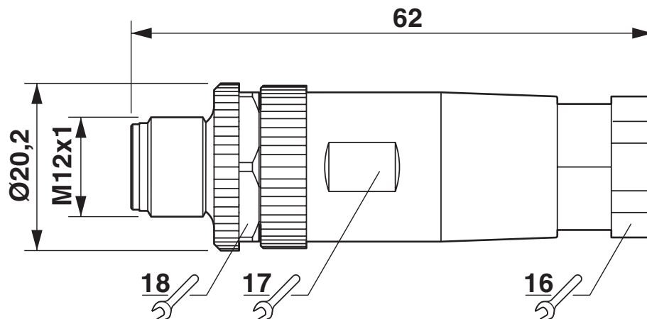
Dimensional drawing
