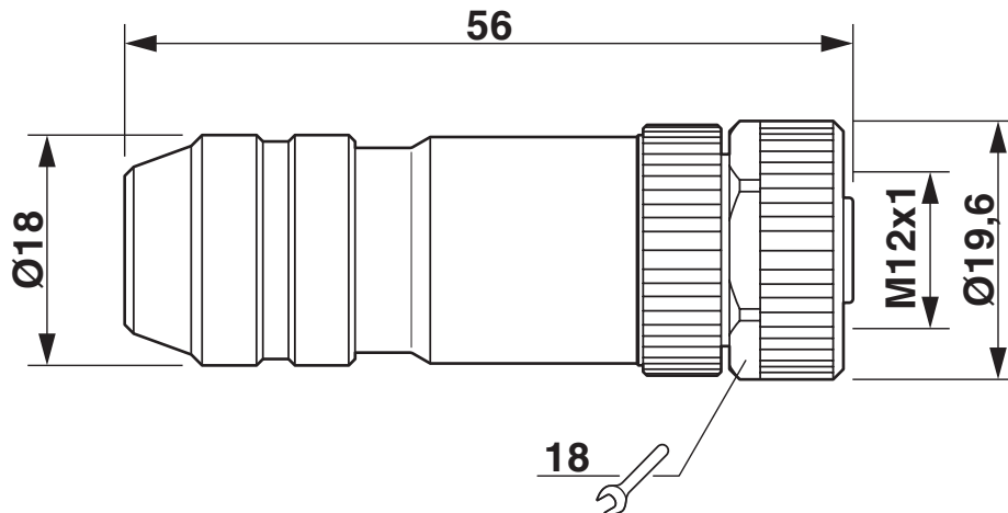
Dimensional drawing
