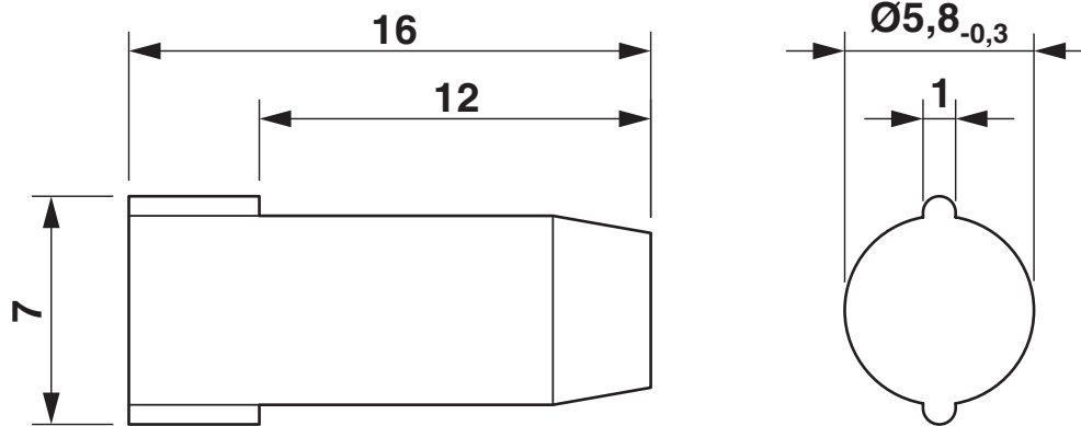
Dimensional drawing
