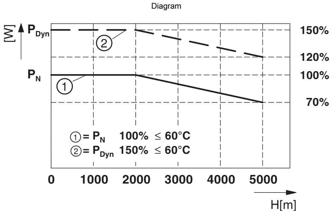
Altitude-dependent derating
