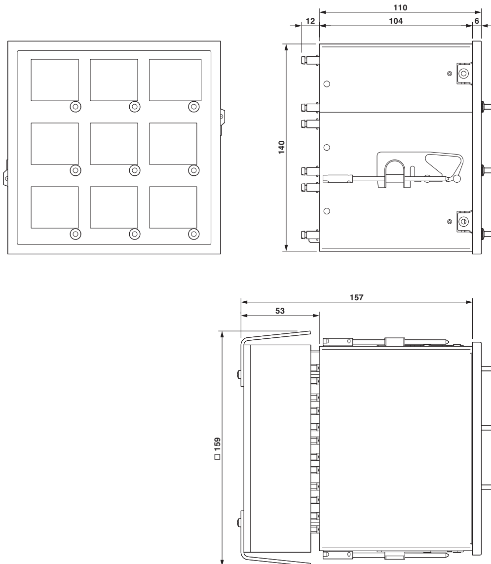
Dimensional drawing
