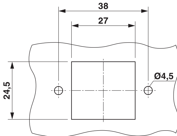
Dimensional drawing
