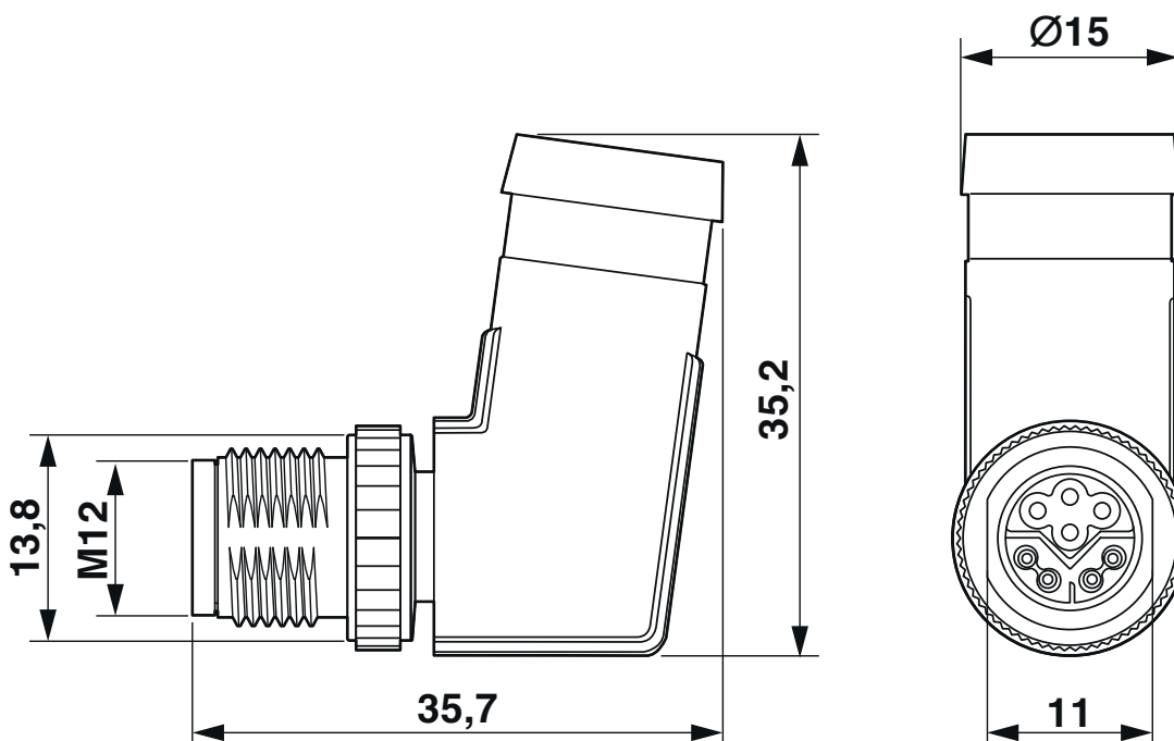
M12 x 1 socket, angled, shielded
