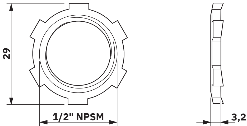
Dimensional drawing
