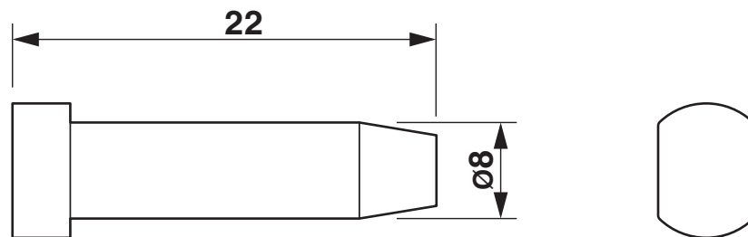
Dimensional drawing
