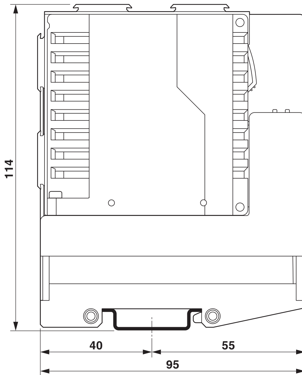
Dimensional drawing
