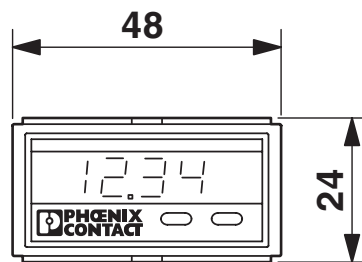
Dimensional drawing
