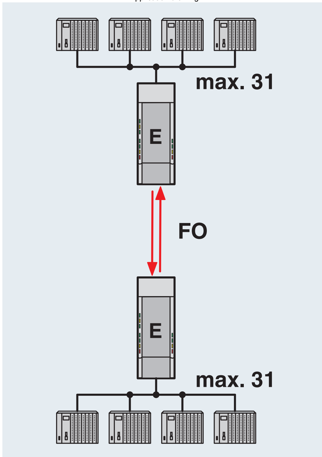
Point-to-point connection
