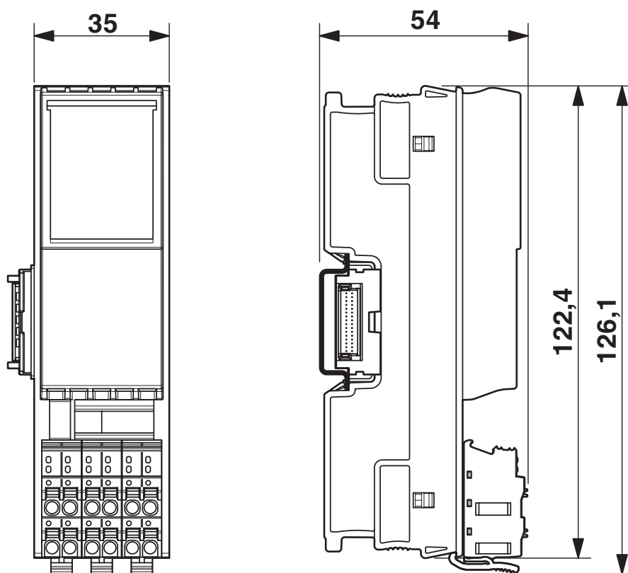
Dimensional drawing
