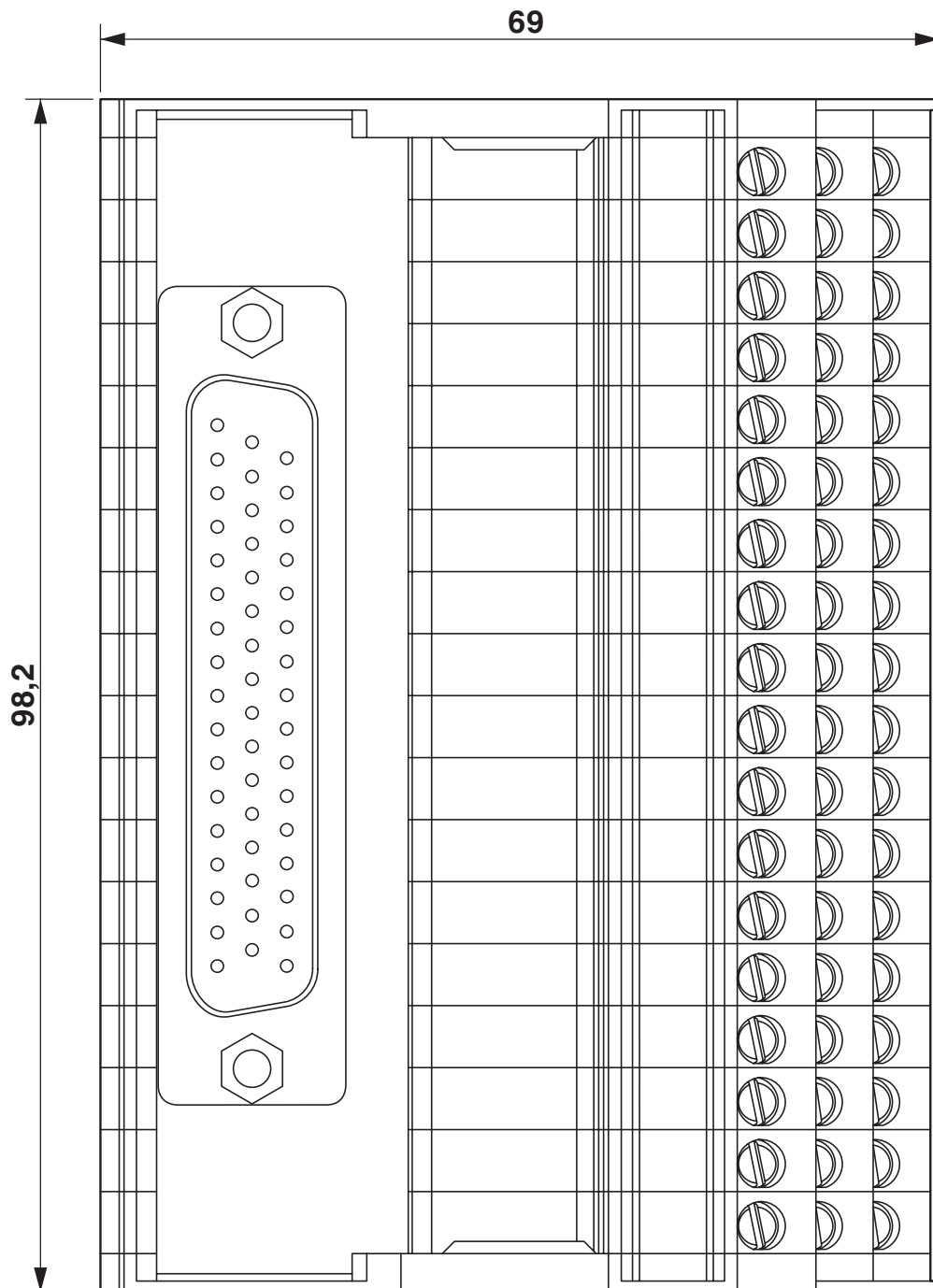
Dimensional drawing
