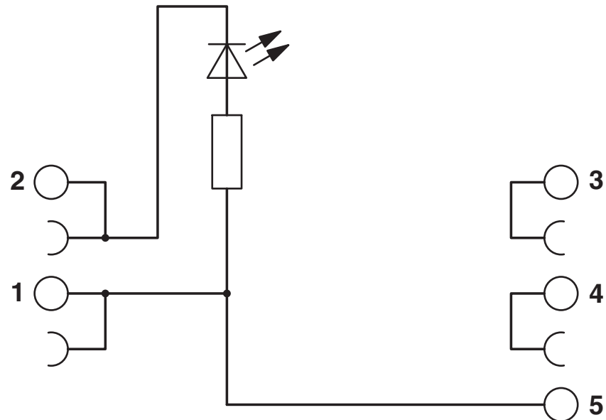
Circuit diagram
