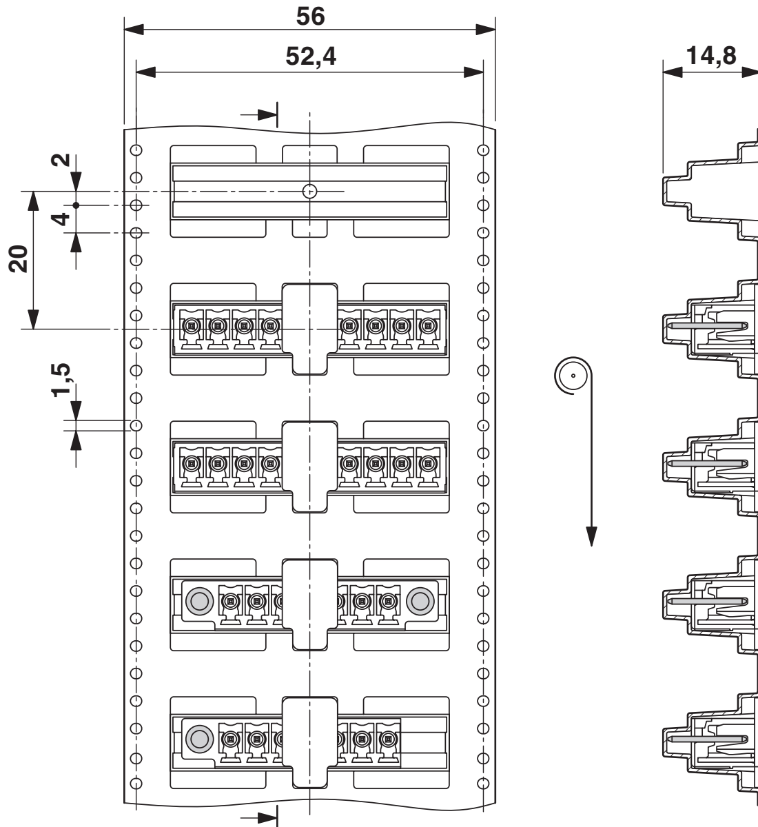
Dimensional drawing
