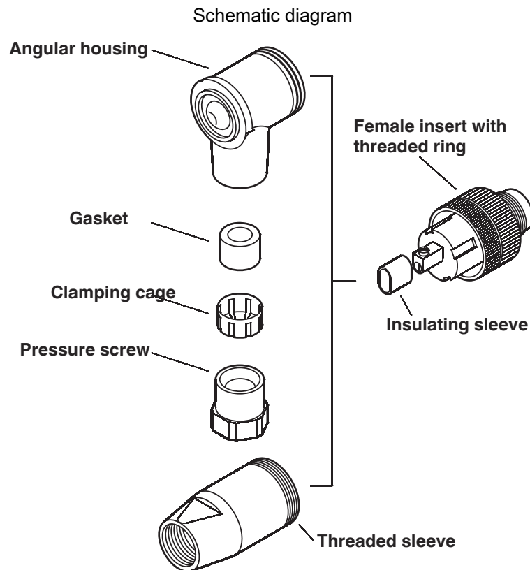
Schematic diagram
