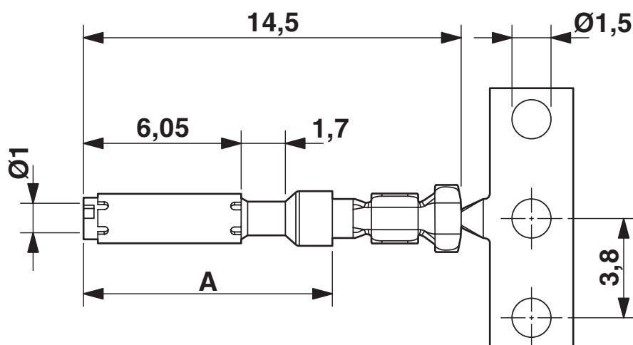
Dimensional drawing
